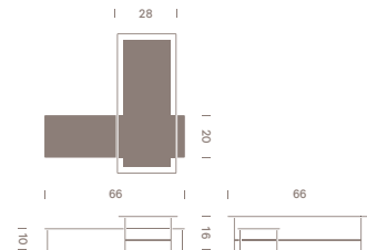
Layer Occasional Table, Nesting
