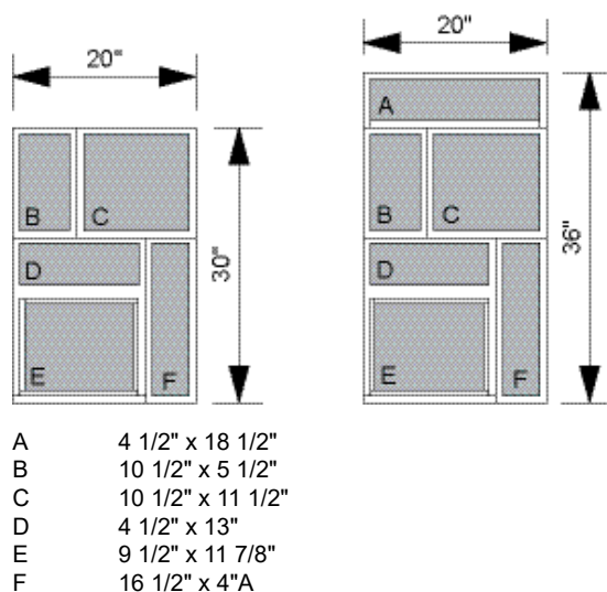
Drawer Dimensions
